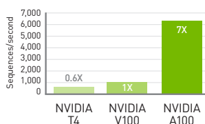
BERT Large Inference
