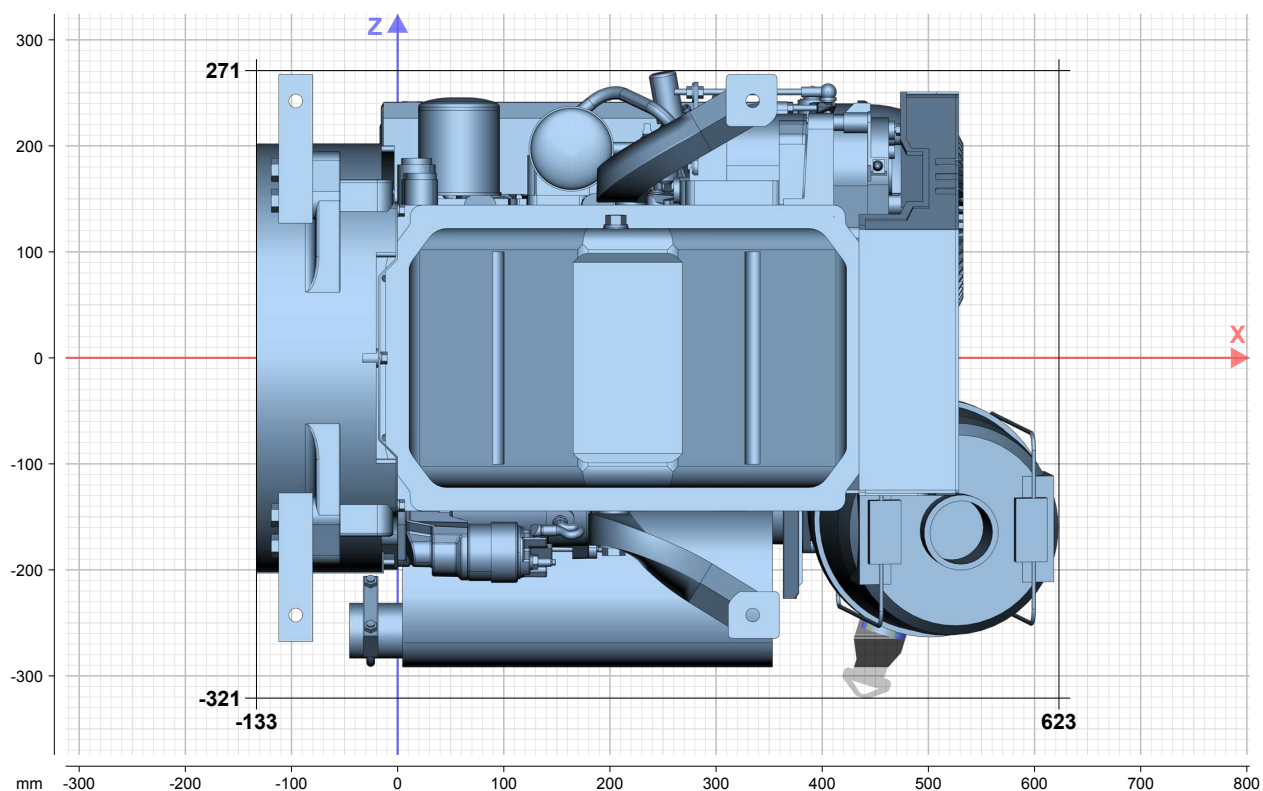
Bottom view
