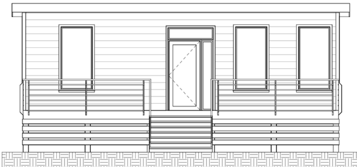
① NORTH ELEVATION
