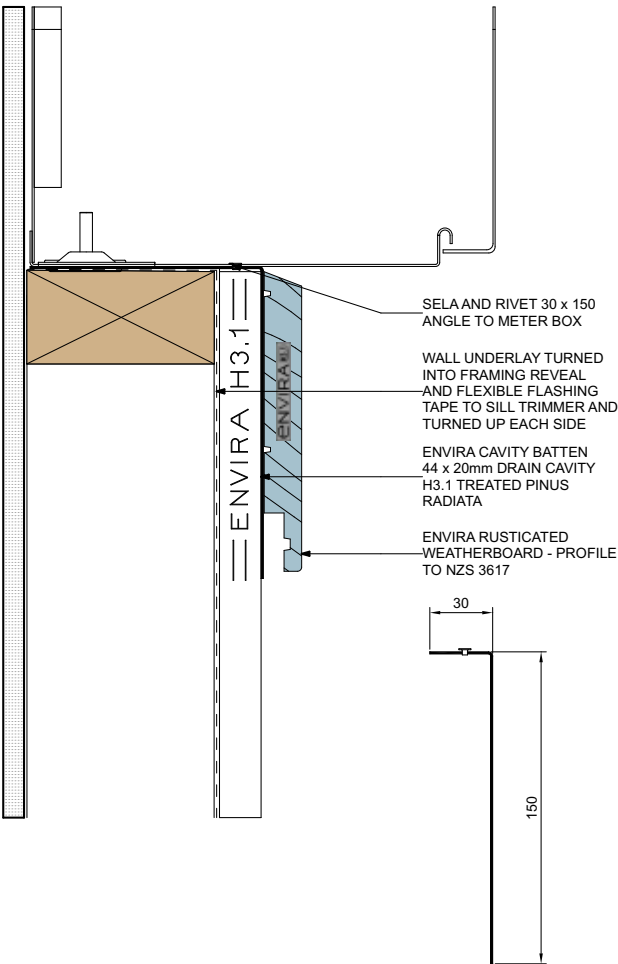
FLASHING DIMENSIONS
