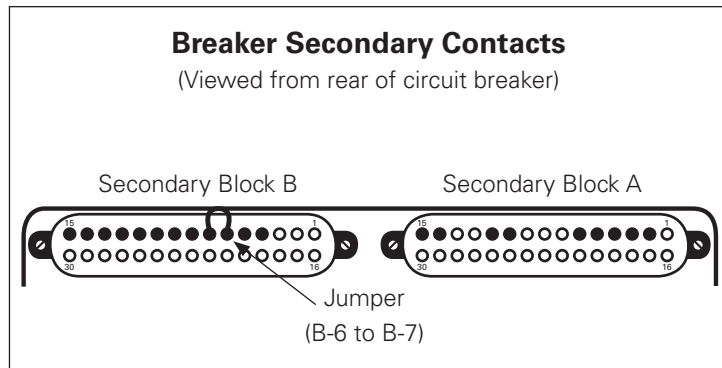
Figure 9. Breaker Secondary Contact Jumper for Ground Fault Test (Magnum)
