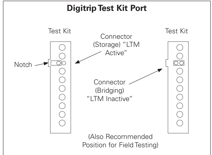
Figure 7. Long Time Memory (LTM) Jumper
