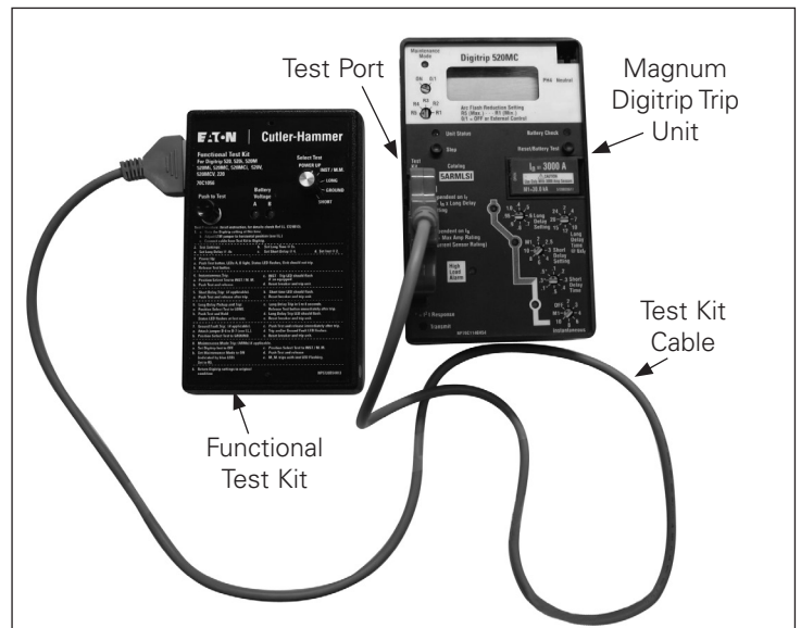
Figure 8. Test Kit and Magnum Digitrip Trip Unit Shown Connected
