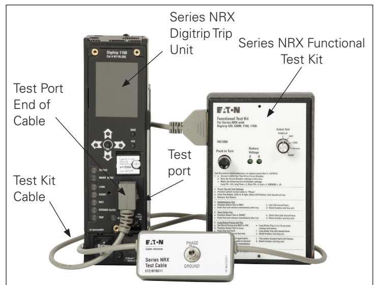
Figure 5. Test Kit and Series NRX Trip Unit Shown
