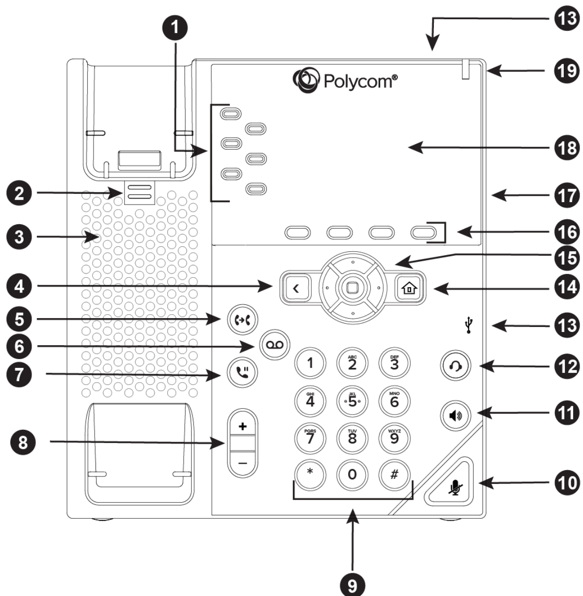
Figure 1. VVX 350 hardware features
