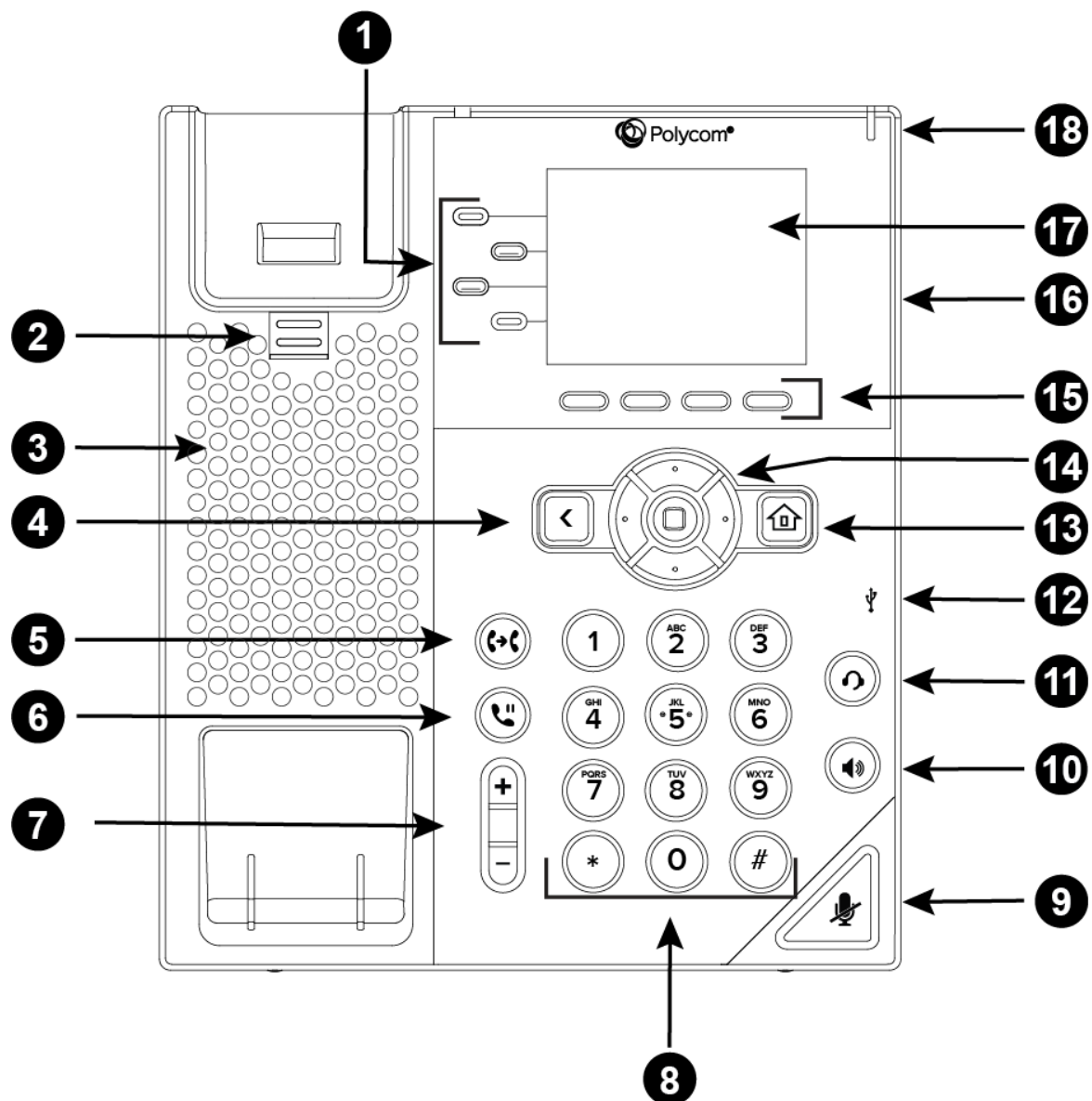
Figure 1. VVX 250 hardware features
