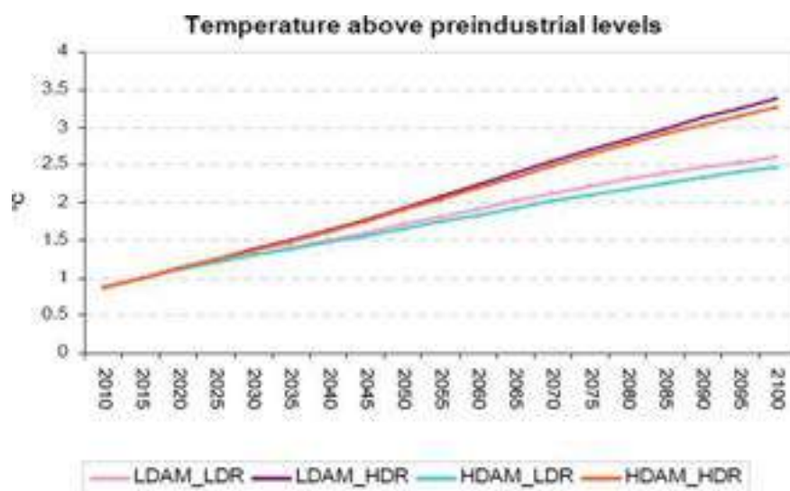
Fig. 14.2 Temperature pathways for low and high damage scenarios
