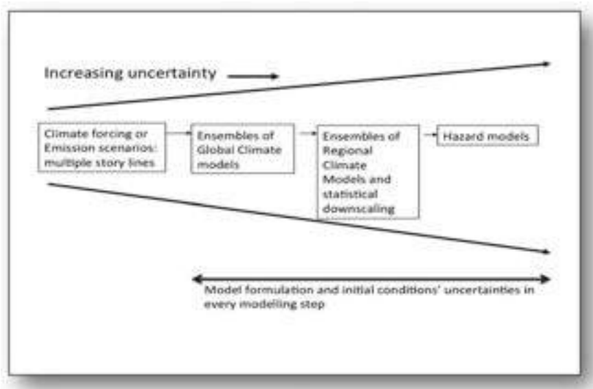
Fig. 11.1 The uncertainty cascade in the modelling chain from climate model forcings to the estimation of the climate hazard (the physical impact of climate change). An estimation of the total risk should include vulnerability and exposure scenarios that, in combination with the climate hazard as inputs for an impact model, outputs the total impact on, for instance, lives, livelihoods, health, ecosystems, economies, societies, cultures, services, and infrastructure
