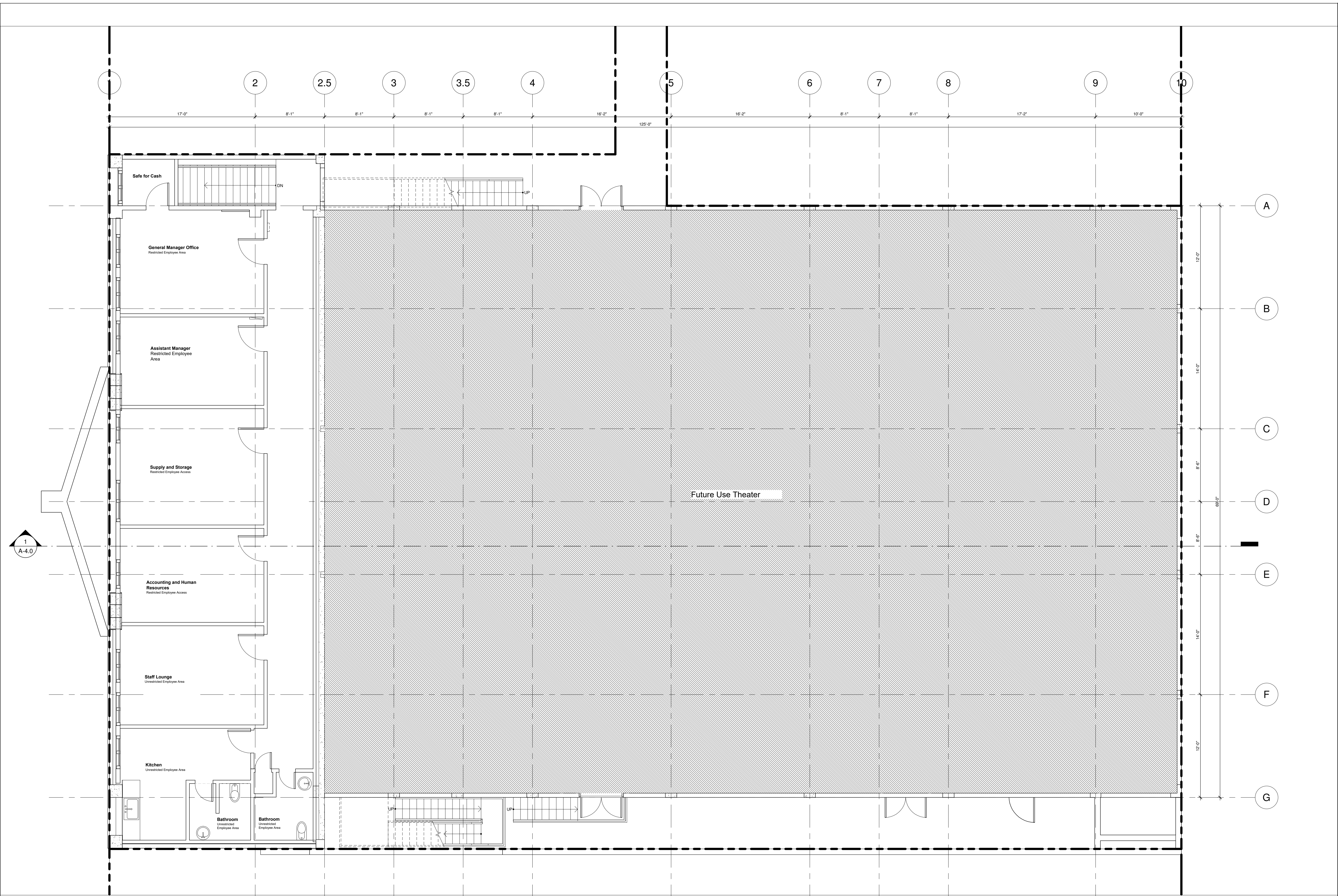
1 (E) LEVEL 2 OFFICE 3/16" = 1'-0"
