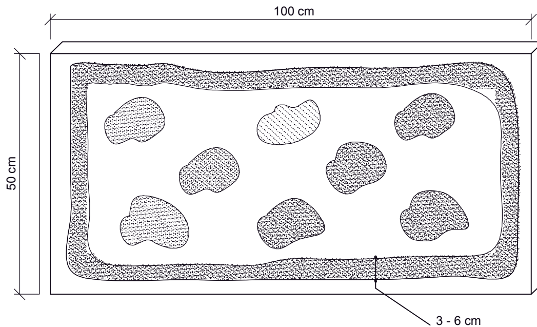
full - surface method (with notched trowel 10 - 12 mm)
