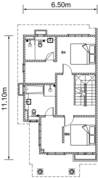
2 nd Floor
