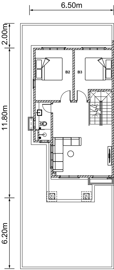
1 st Floor
