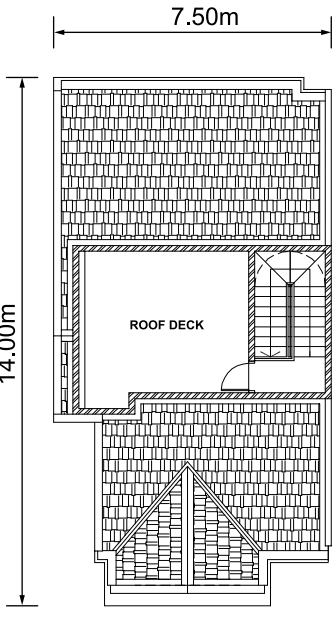
Roof
