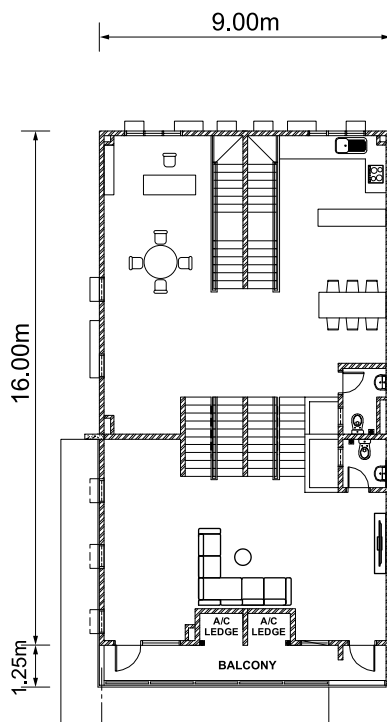
1 st Floor
