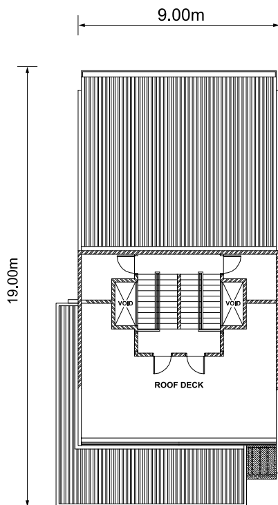
Lower Roof
