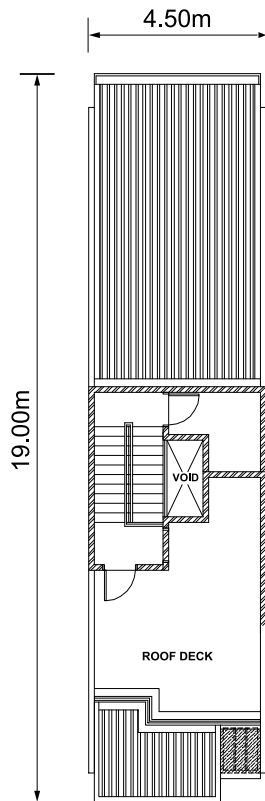
Lower Roof
