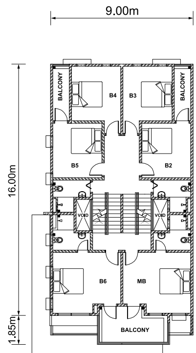
2 nd Floor
