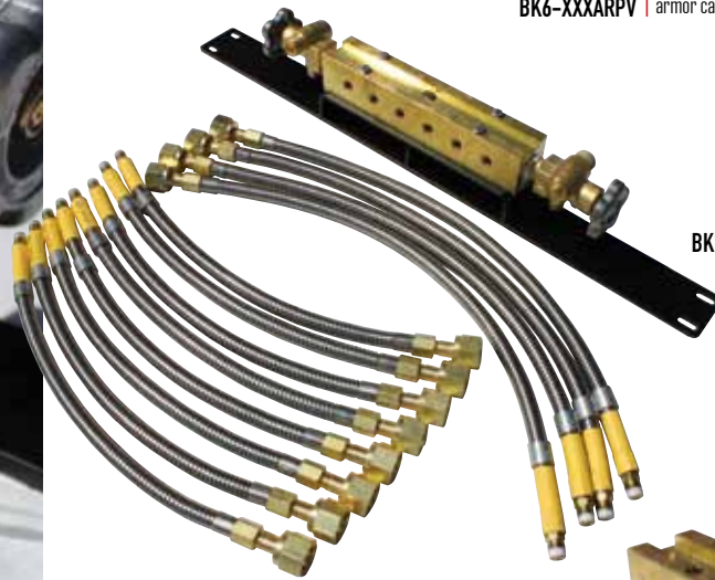
Part Number BK6-XXXARPV | 6 cylinder block manifold system with post sintered, armor cased pigtails and RPV valves
