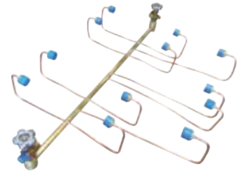
Part Number | Brass manifold with copper pigtails, 912-XXXIN | Overhang design for Zeus & Titan cradles
