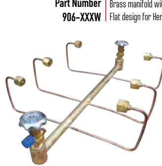
Part Number 906-XXXIN | Brass manifold with copper pigtails, Overhang design for Zeus & Titan cradles
