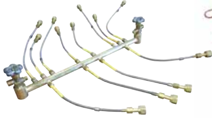
Part Number | Brass manifold with post sintered 932-XXXINPS | flexible pigtails and RPV valves
