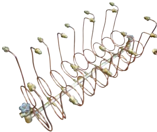
Part Number 9118-XXX | Brass manifold with replaceable copper pigtails
