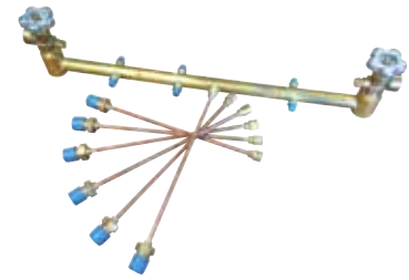
Part Number 916-XXXST | Brass manifold with replaceable copper pigtails, Flat design for top mount Brut cradles
