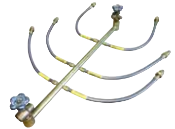
Part Number 926-XXXINARPV | Brass manifold with armor cased post sintered flexible pigtails and RPV valves
