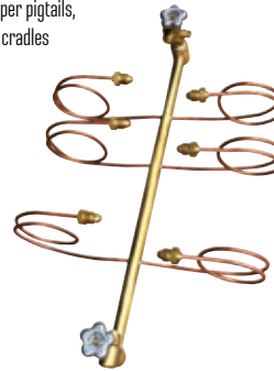
Part Number 906SL-XXXINRPV | Brass manifold with single loop copper pigtails and RPV valves, Overhang design for Zeus & Titan cradles
