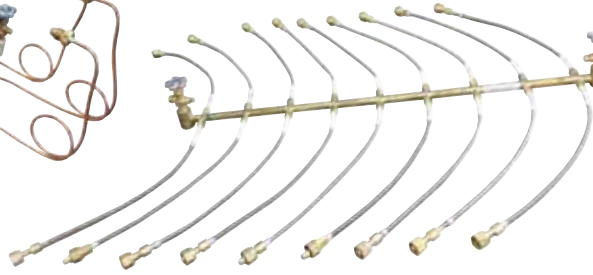
Part Number 9218-XXX | Brass manifold with flexible pigtails
