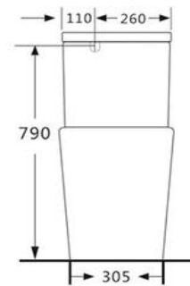
Frontal view
