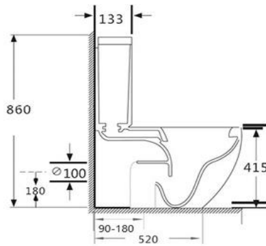
Sid view
