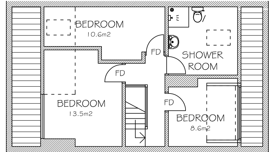
ATTIC
