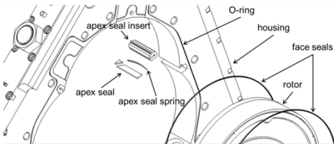
Figure 6 Main gas sealing components of X1 engine
