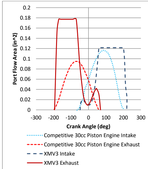
Figure 15 Intake and Exhaust porting / minimum restriction area in XMv3 compared to a Competitive SI single cylinder 30cc engine.
