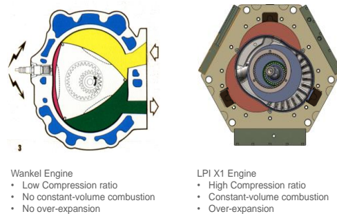
Figure 7 Comparison of LiquidPiston X architecture and Wankel
