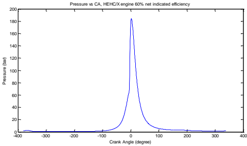
Figure 2: Firing pressure trace from the 0D model, X1, full load, 1800rpm, and indicated efficiency 60%, peak pressure of 190bar
