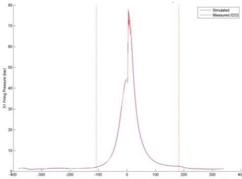
Figure 11 firing trace of X1 test results (red) and the 0D model comparison, 1800rpm, 50% load. Pressure (bar) vs CA (degrees). Red dashed lines show intake port closing (IPC) (left) and exhaust port open (EPO) (right).
