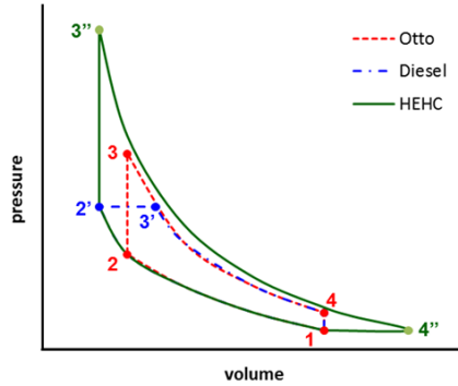
Figure 1 p-V diagram comparing ideal air-standard cycles
