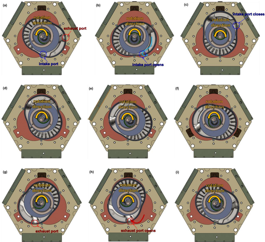
Figure 5 Operation of X1 engine: (a) just before intake port opens, (b) intake stroke starts, (c) intake stroke completes, (d) compression stroke starts, (e) compression stroke completes and combustion occurs, (f) expansion stroke starts, (g) expansion stroke completes, (h) exhaust stroke starts, and (i) exhaust stroke completes
