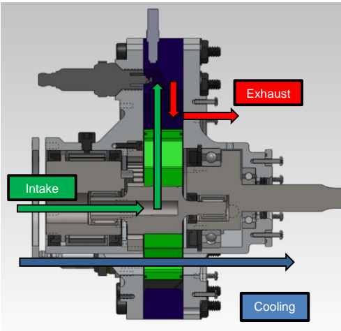
Figure 13 XMv3 section view and flow configuration
