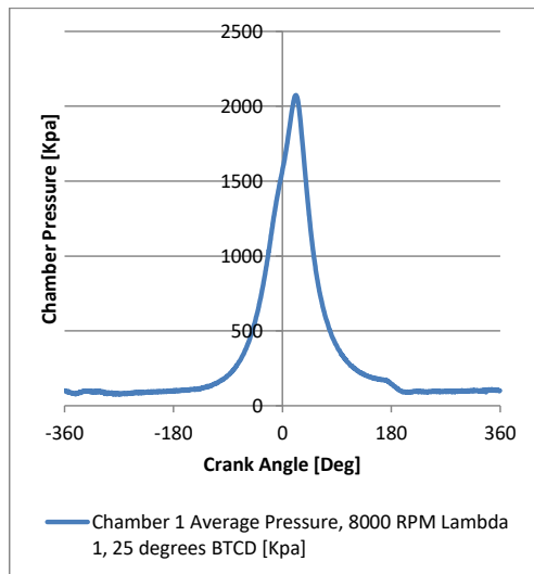
Figure 17 Firing trace for XMv3, SI, 8000 rpm full load
