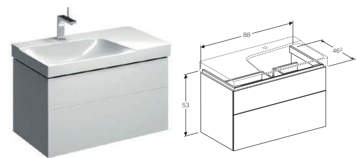
Cabinet for 90cm washbasin, with two drawers W 88 / D 46.2 / H 53cm
