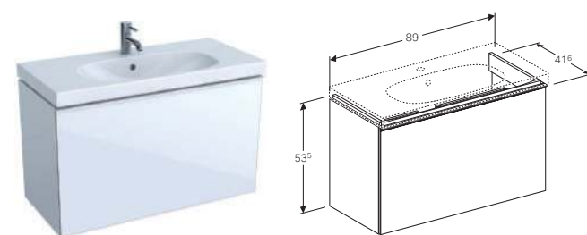
Cabinet for 90cm washbasin, with one drawer and internal drawer, small projection W 89 / D 41.6 / H 53.5cm
