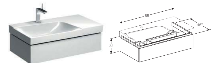
Cabinet for 90cm washbasin, with one drawer W 88 / D 46.2 / H 22cm
