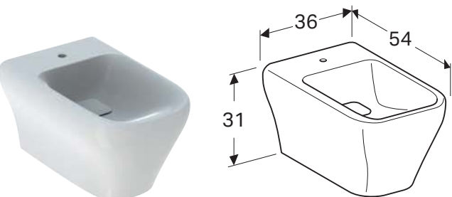
Wall hung bidet W 36 / D 54 / H 31cm Hidden water supply connection, hidden fastening. Art. no. 235450600
