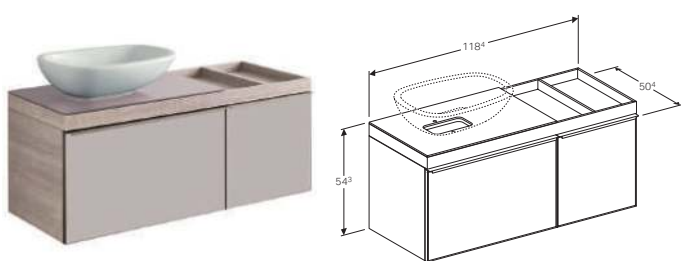
120cm cabinet for lay-on washbasin, with two SoftClosing mechanism drawers and shelf surface W 118.4 / D 50.4 / H 54.3cm
