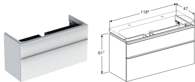
Cabinet for 120cm handrinse basin, with two SoftClosing mechanism drawers W 116.8 / D 49 / H 62.5cm
