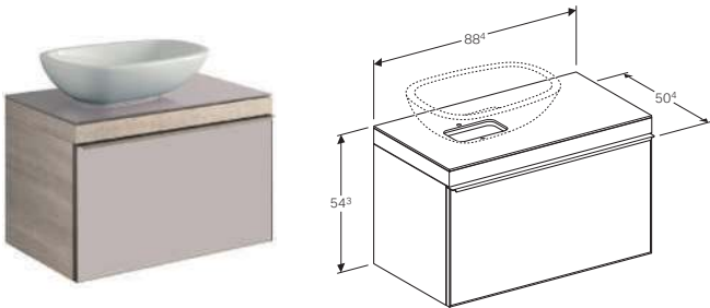
90cm cabinet for lay-on washbasin, with one SoftClosing mechanism drawer W 88.4 / D 50.4 / H 54.3cm
