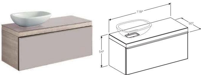
120cm cabinet for lay-on washbasin, with one SoftClosing mechanism drawer W 118.4 / D 50.4 / H 54.3cm
