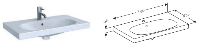
75cm washbasin, small projection, shelf surface W 74.5 / D 42.2 / H 5.5cm
