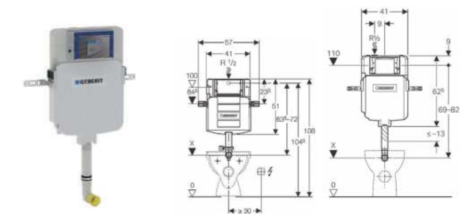
Geberit Sigma concealed cistern, 6/3 litres
