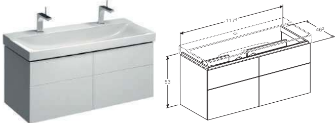
Cabinet for 120cm washbasin, with four drawers W 117.4 / D 46.2 / H 53cm
