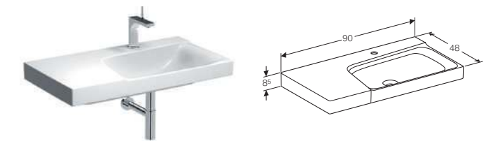
90cm washbasin with shelf surface W 90 / D 48 / H 8.5cm
