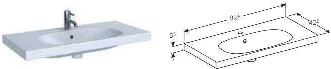
90cm washbasin, small projection, shelf surface W 89.5 / D 42.2 / H 5.5cm
