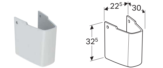
Semi pedestal W 22.5 / D 30 / H 32.5cm Not suitable for 60cm countertop basin. Art. no. 291410600
