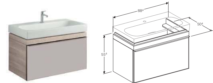
Cabinet for 90cm washbasin, with one SoftClosing mechanism drawer W 88.4 / D 50.4 / H 55.4cm
