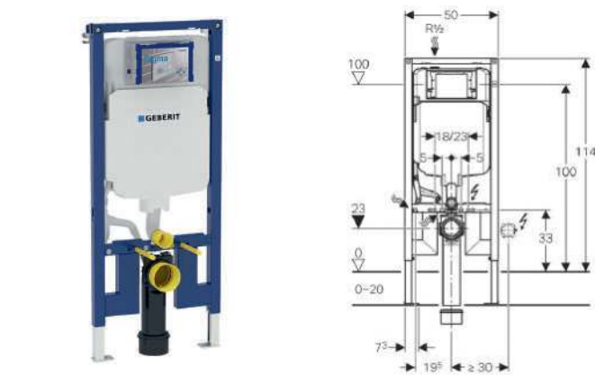
Geberit Duofix WC frame with Sigma cistern 8cm
