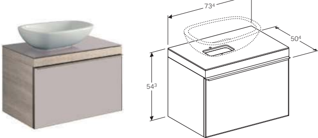
75cm cabinet for lay-on washbasin, with one SoftClosing mechanism drawer W 73.4 / D 50.4 / H 54.3cm
