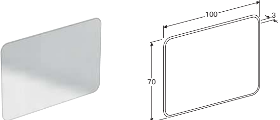
100cm mirror W 100 / D 3 / H 70cm LED lighting, indirect lighting, light operated by wall switch, heated rear to prevent mirror steaming up.
