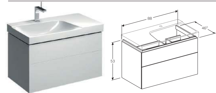
Cabinet for 90cm washbasin, with two drawers W 88 / D 46.2 / H 53cm
