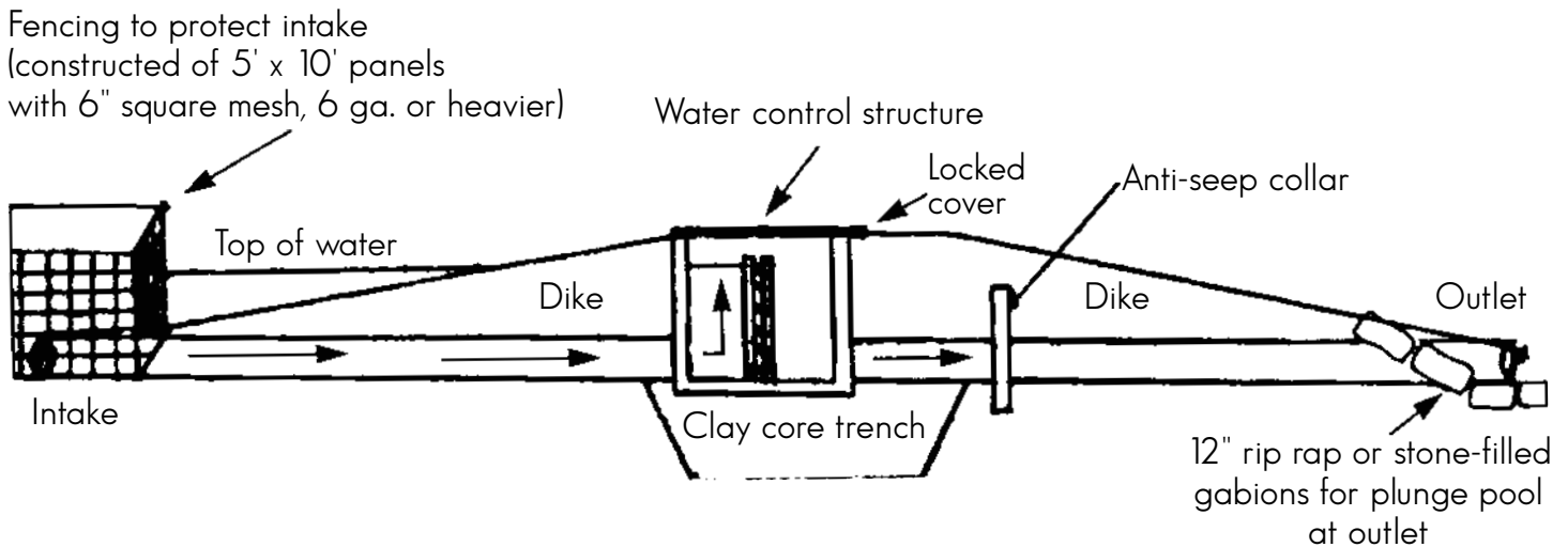
Cross Section of Low Level Dike and Water Control Structure
