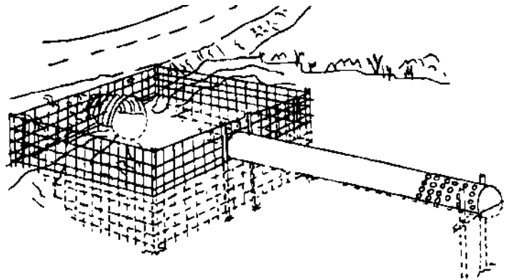
Correct Installation
