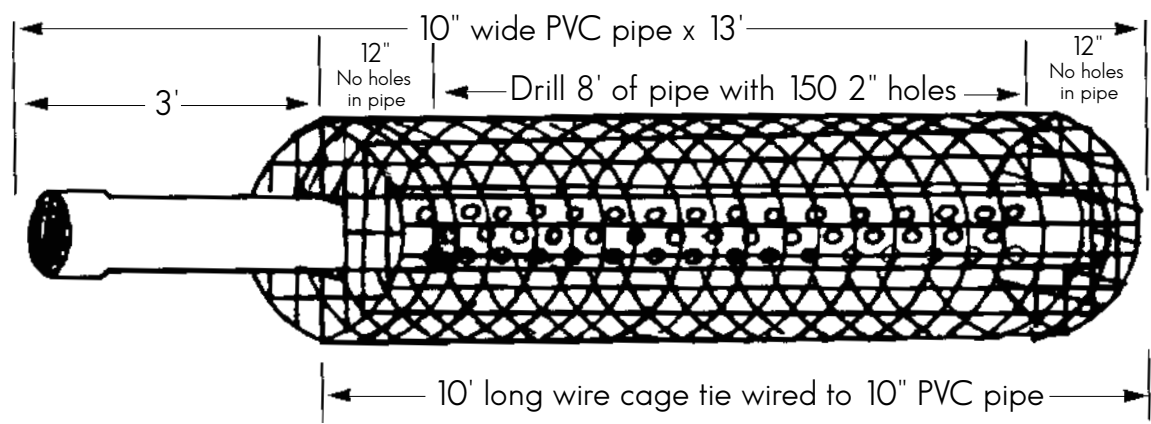
Clemson Intake Device
