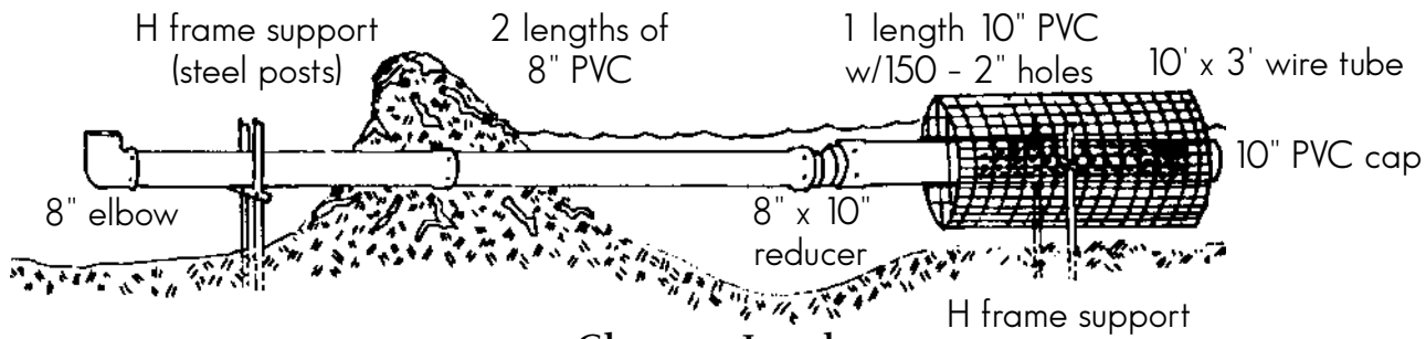
Clemson Leveler
