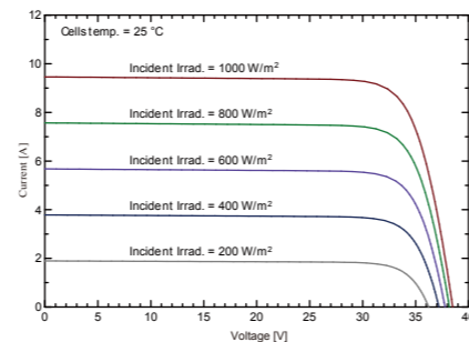
I-V Curve (SRP-290-BMB(-HV))
