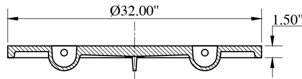
SECTION OF COVER
