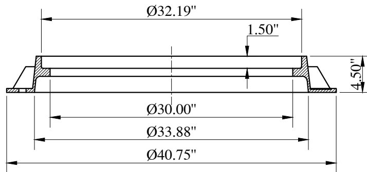
SECTION OF FRAME
