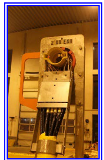
Ubas H with two single MQC / Cobra Head Parking Stands and a 165m long 17cm dia. HFL with double spiral guard.
