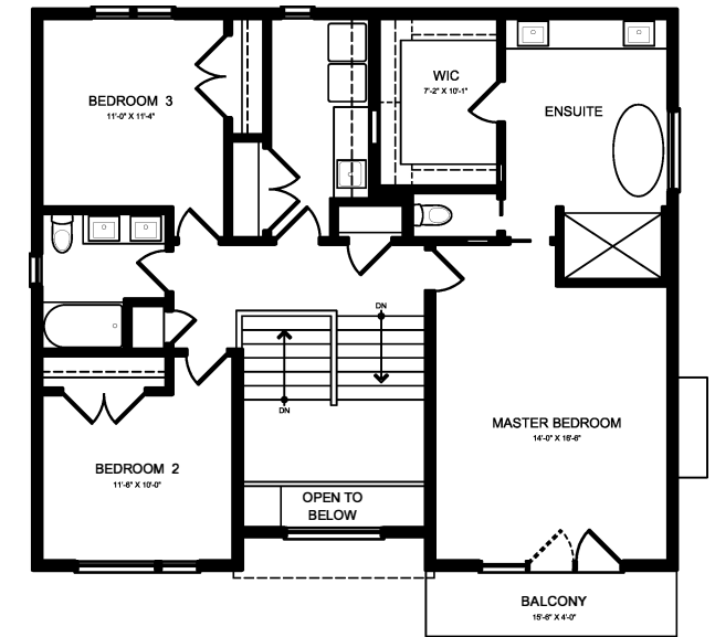
UPPER FLOOR PLAN 1 2 3 5 SQ.FT.
