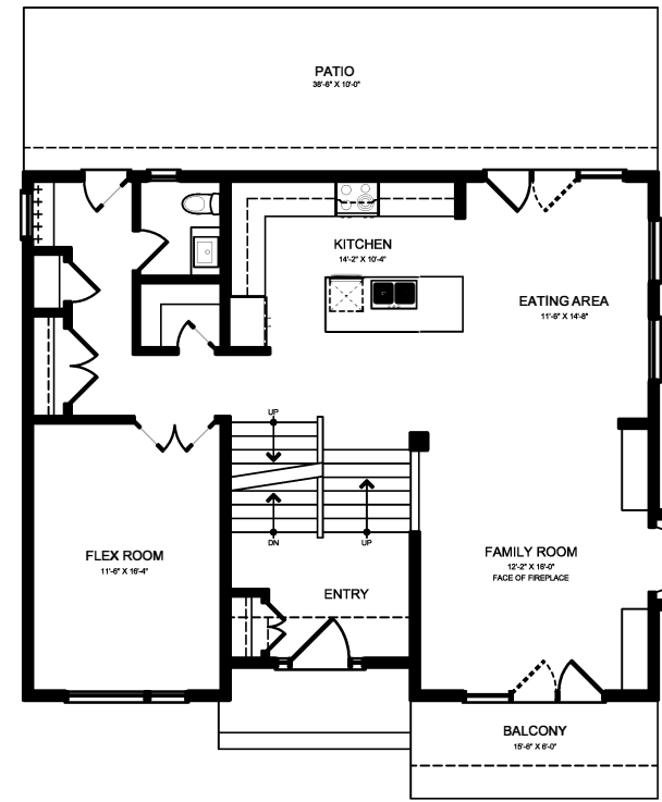
MAIN FLOOR PLAN 1 2 2 1 SQ.FT.
