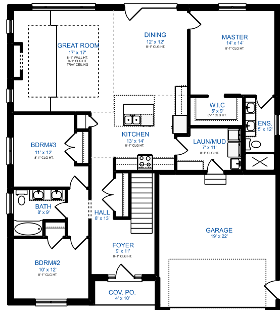
MAIN FLOOR PLAN AREA = 1752.5 Sq.ft
