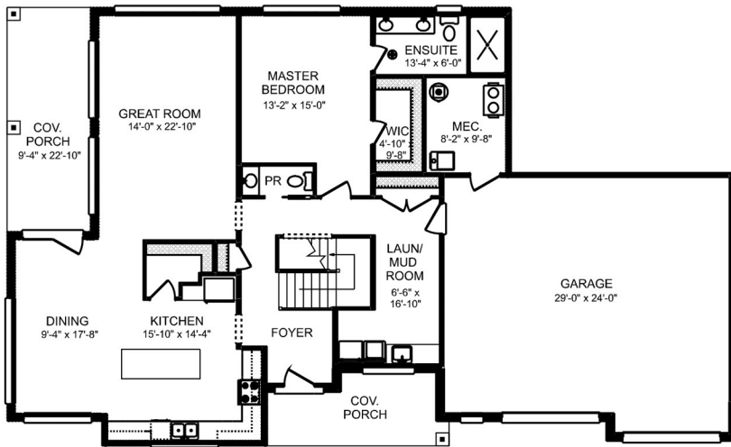
MAIN FLOOR PLAN AREA = 1766 SQ.FT.
