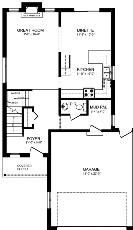
MAIN FLOOR PLAN AREA: 818 SQ.FT.
