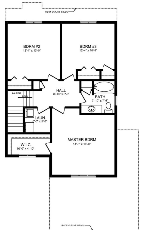
SECOND FLOOR PLAN AREA: 837 SQ.FT.
