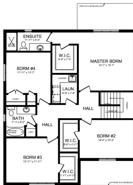
SECOND FLOOR PLAN AREA 1,272 SQ.FT.
