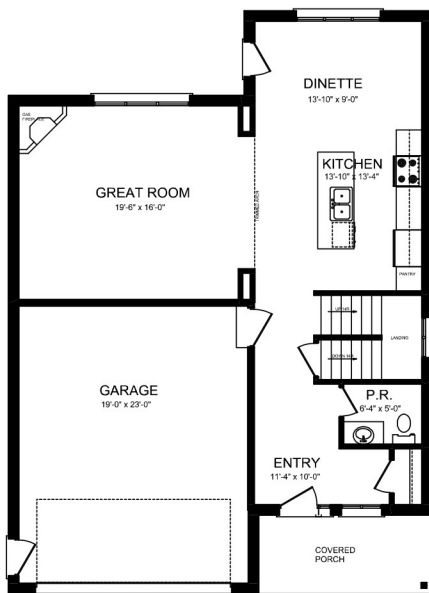
MAIN FLOOR PLAN AREA 978 SQ.FT.
