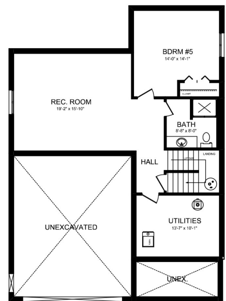
BASEMENT PLAN AREA 815 SQ.FT.
