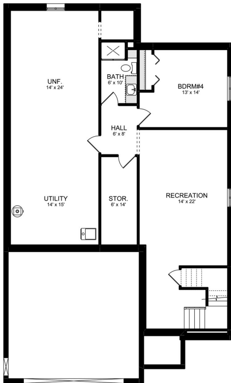
BASEMENT FLOOR PLAN FINISHED AREA = 665 Sq.ft.
