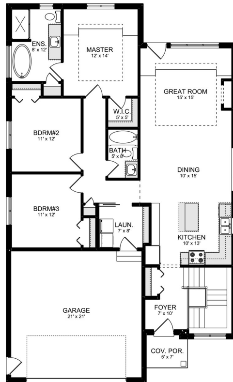
MAIN FLOOR PLAN AREA = 1614 Sq.ft.
