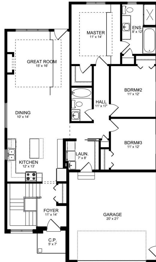
MAIN FLOOR PLAN AREA = 1524 SQ.FT. TOTAL LENGTH x WIDTH 60'-10" x 35'-8"
