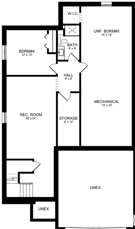
BASEMENT FLOOR PLAN FINISHED AREA = 618 SQ.FT. TOTAL LENGTH x WIDTH 60'-10" x 35'-8"
