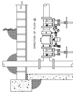
VERTICAL INSTALLATION
