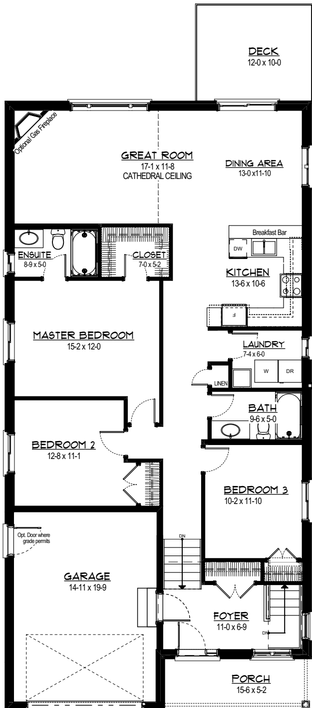
3 Bedroom Floor Plan
