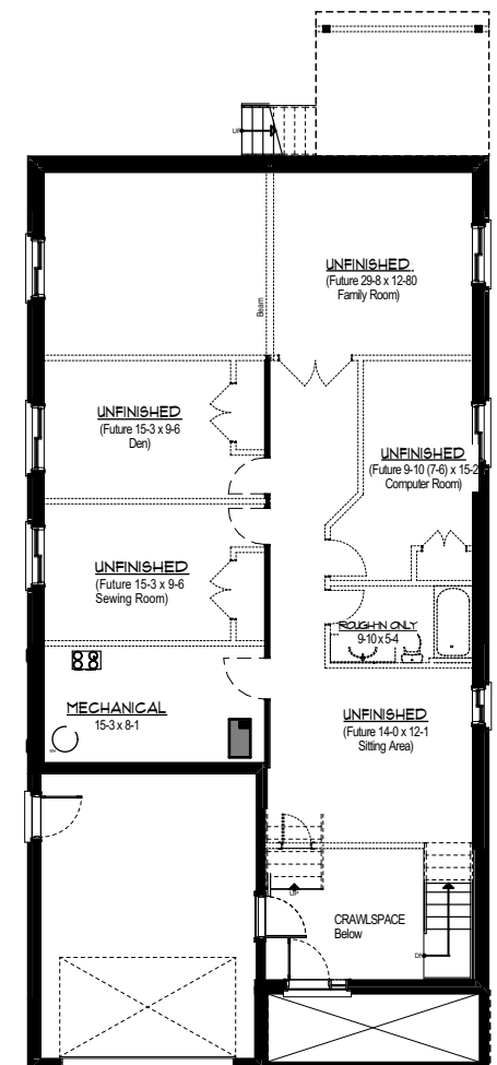
Basement Plan
