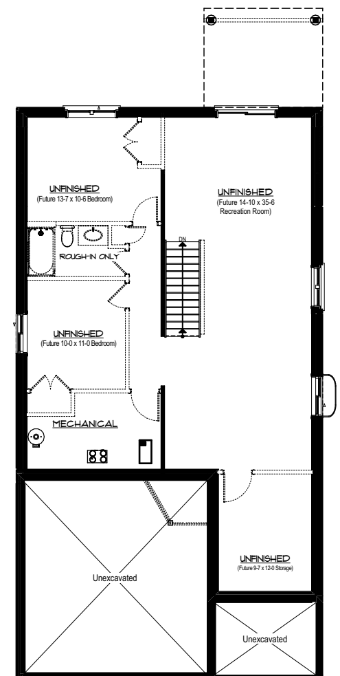
Basement Area = 1,312 sq ft Basement Plan
