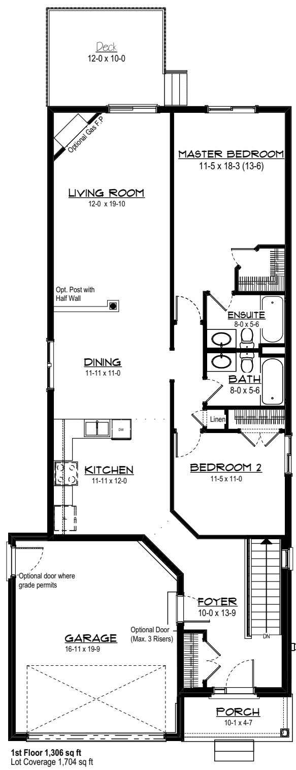
1st Floor 1,306 sq ft Lot Coverage 1,704 sq ft 1st Floor Elevation B/C with Optional Ensuite
