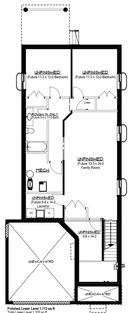
Finished Lower Level 1,113 sq ft Total Lower Level 1,320 sq ft Basement Elevation B/C
