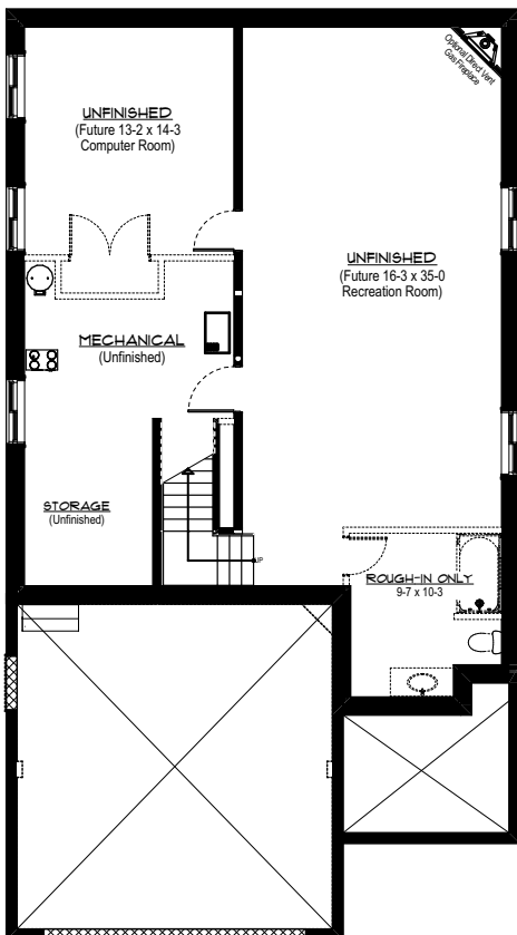
Basement Plan
