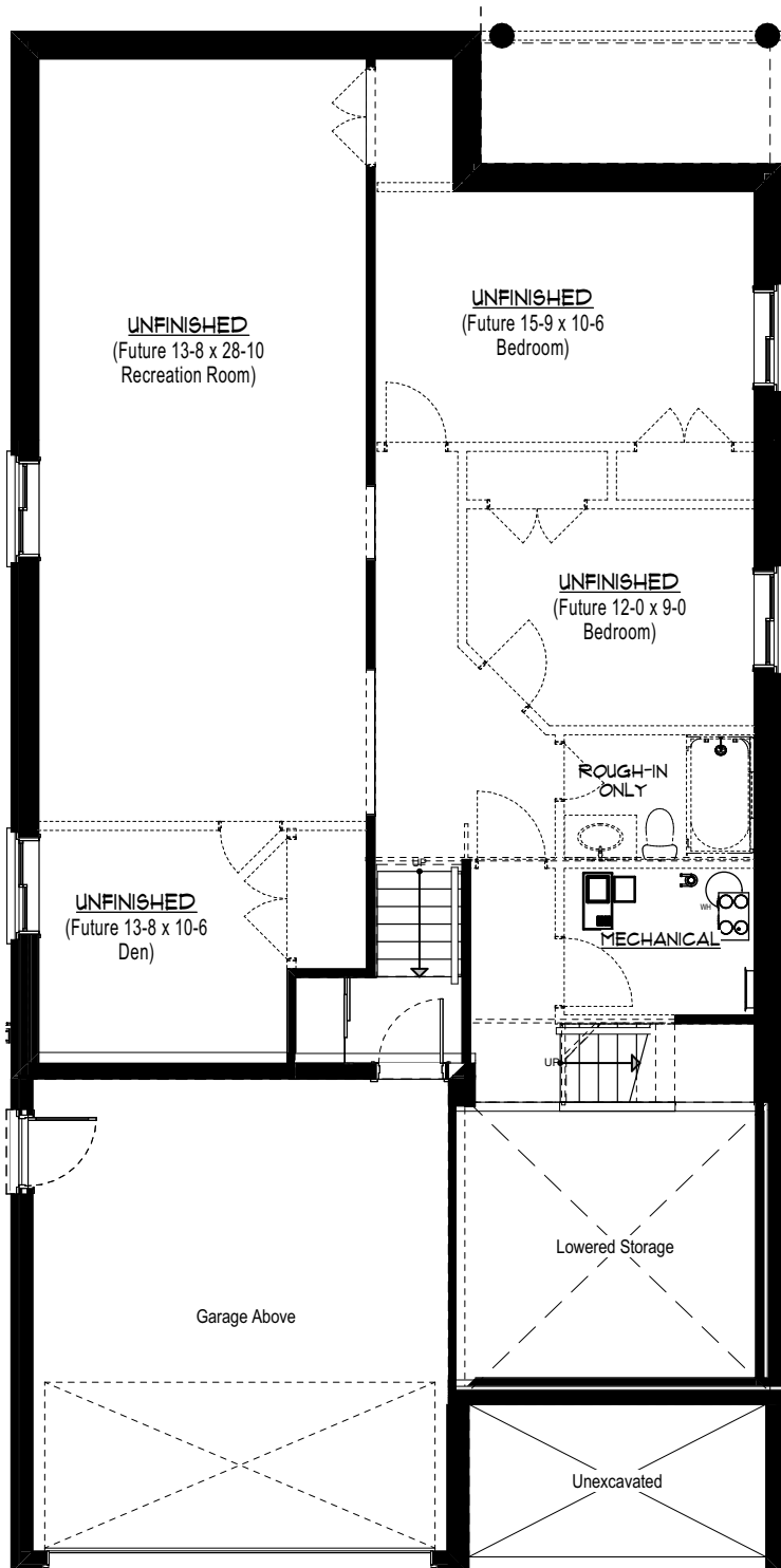
Basement Plan
