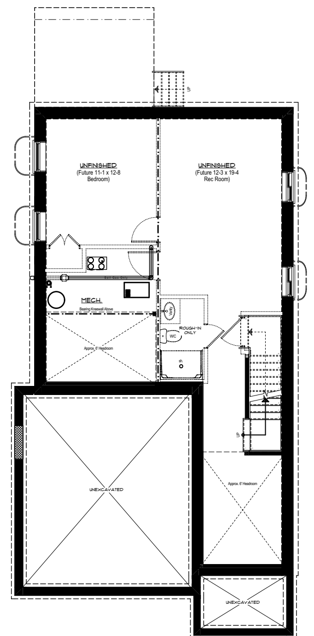
Basement Plan
