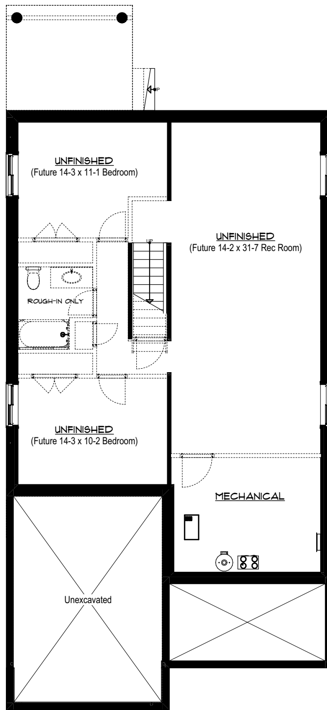
Basement Plan
