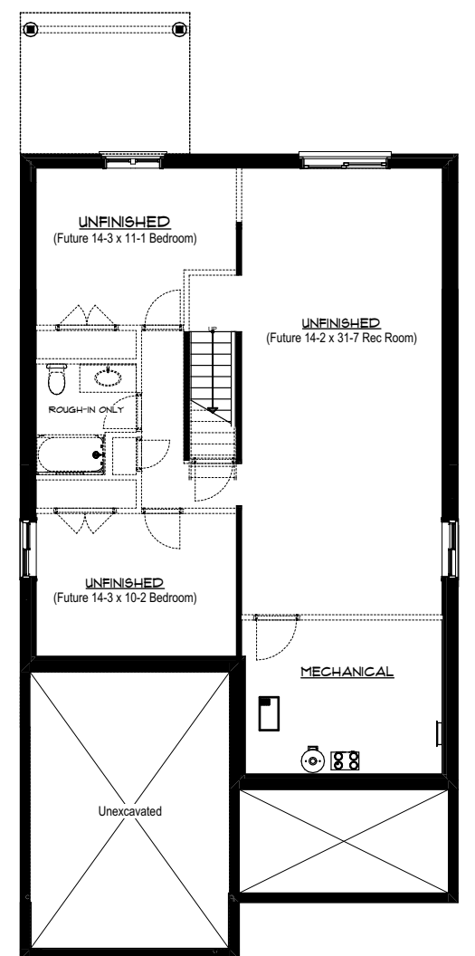
Optional Basement Walk-out (Specific Lots where Grade Permits)
