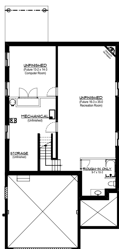
Basement Plan
