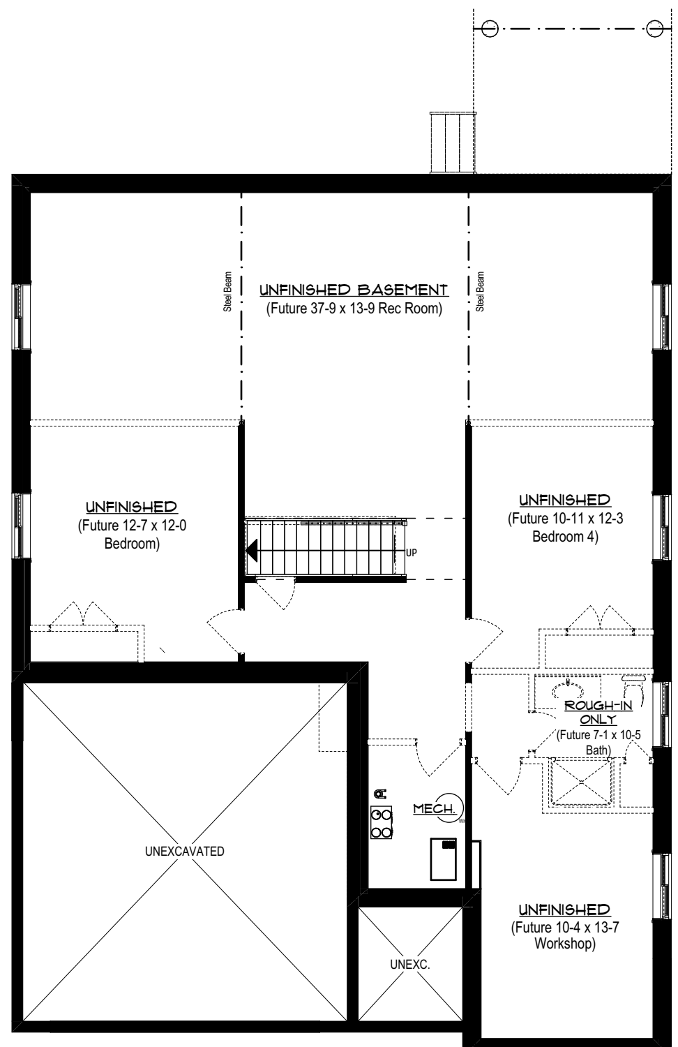
Basement Plan
