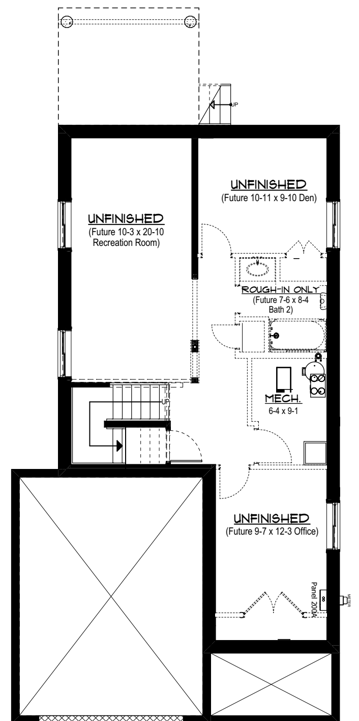
Basement
