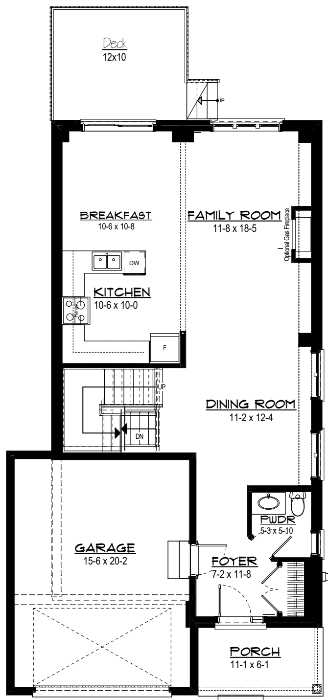
1st Floor
