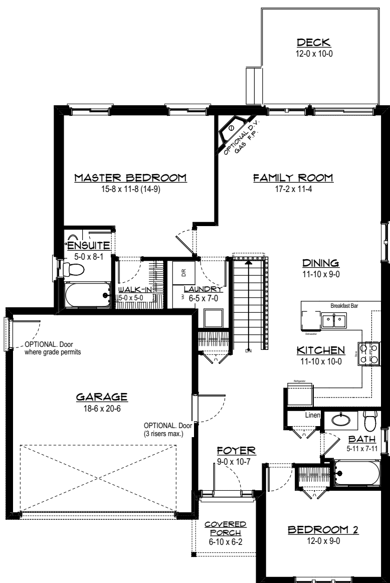
1st Floor Plan Elevation A
