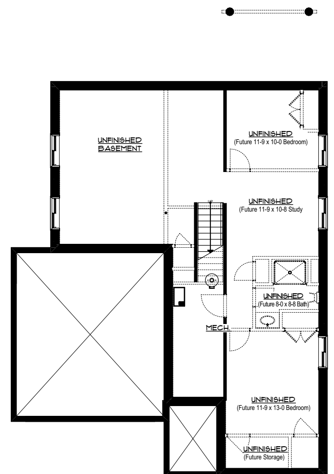
Basement Plan
