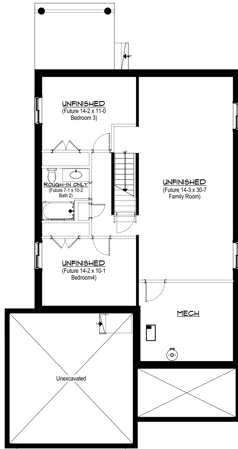
Basement Plan
