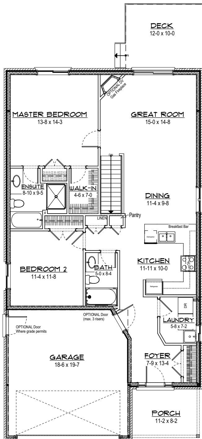
1st Floor Plan 2 Bedroom
