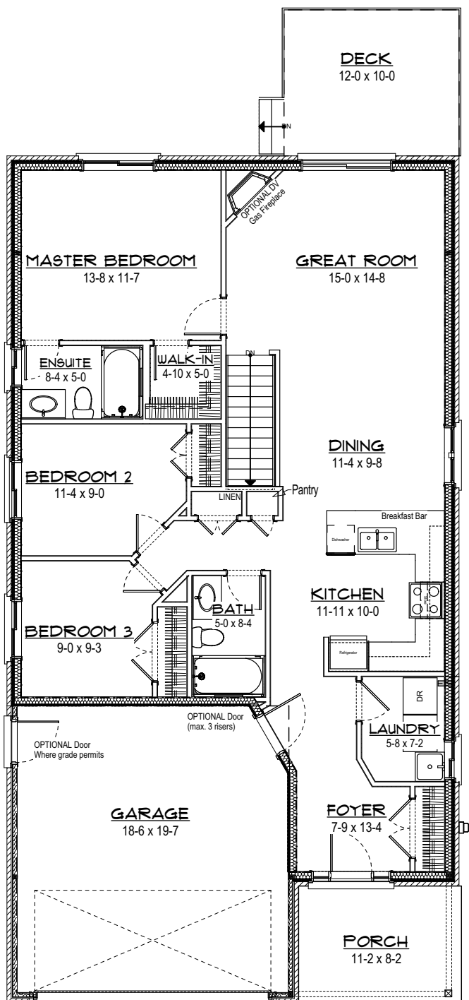
1st Floor Plan 3 Bedroom
