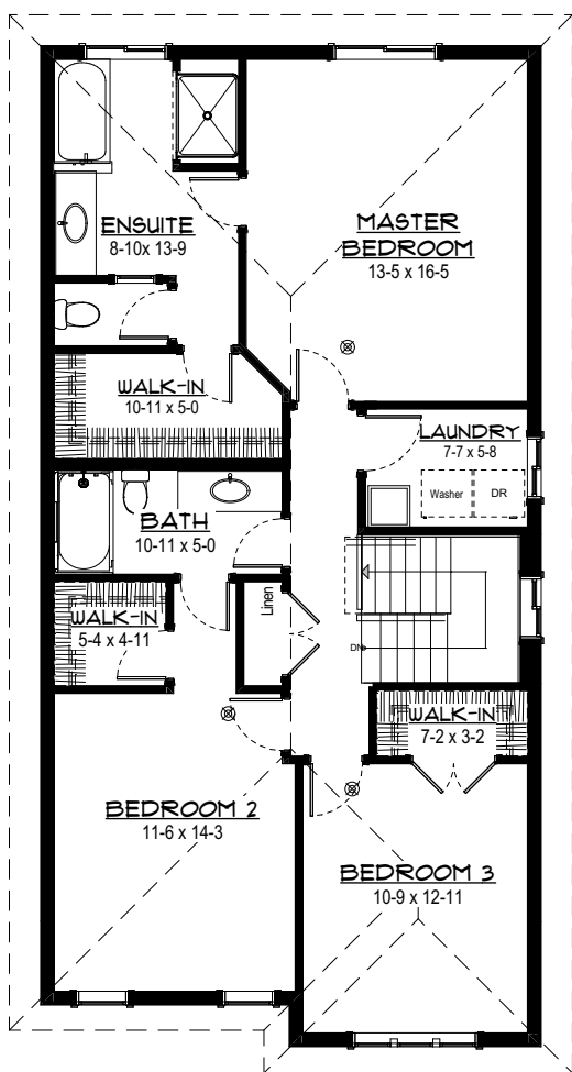
2nd Floor 3 Bedroom
