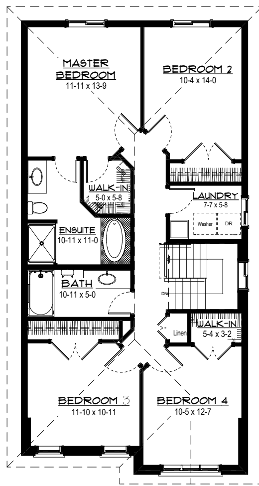
2nd Floor 4 Bedroom
