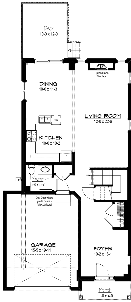
1st Floor
