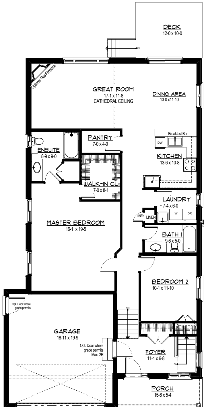
2 Bedroom Floor Plan
