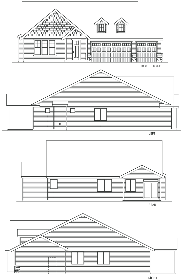
Lot 30 - elevation / floor plan drawings
