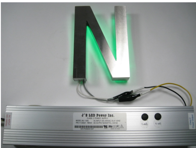
5. Connect to 12 V DC power supply.
