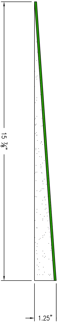
Side View
