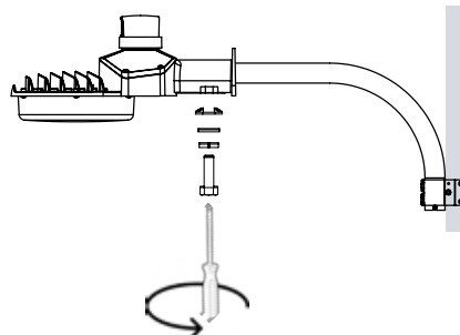
Extension Arm Mount
