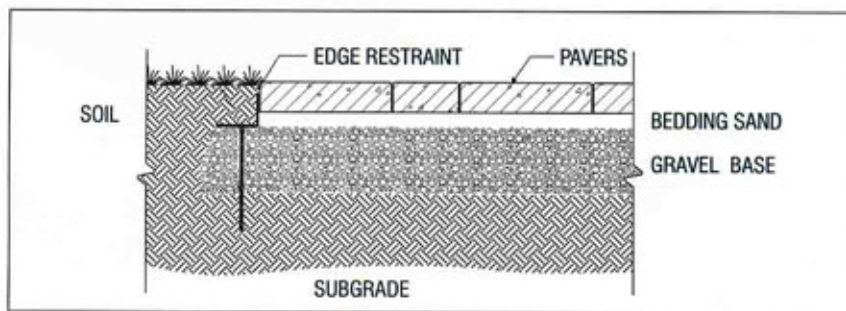
Typical Cross Section - for more information, see Unilock Paver Specifications.
